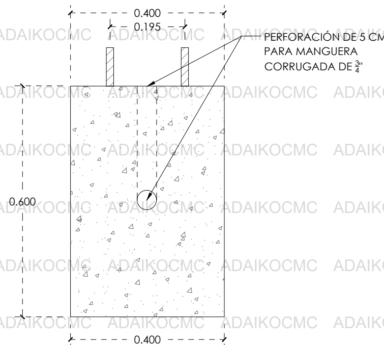
VISTA FRONTAL
