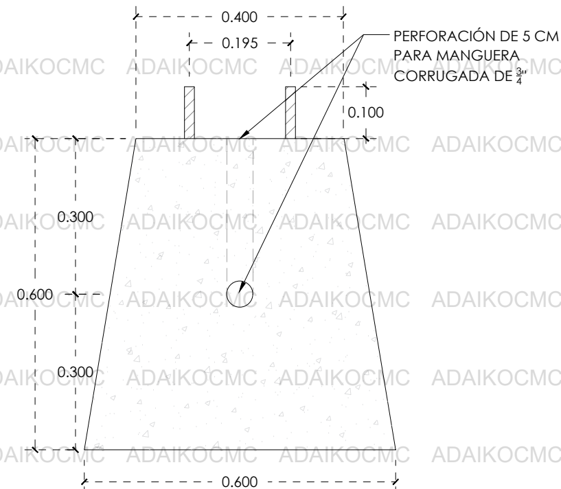
VISTA FRONTAL
